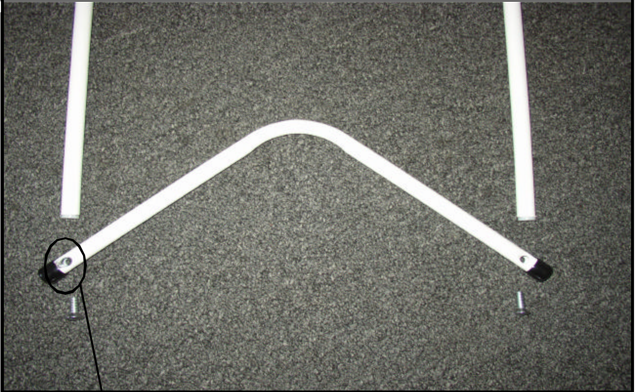
Assemble stand with dimpled holes facing outward
